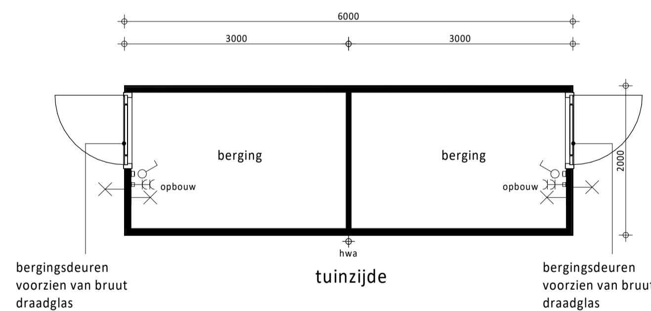
Plattegrond (type 3)
