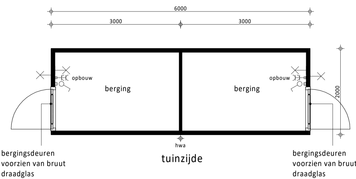
Plattegrond (type 2)
