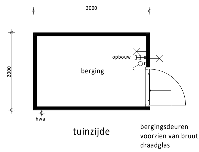
Plattegrond (type 1)
